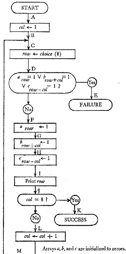
Fig. 2. Nondeterministic algorithm for the eight queens problem
